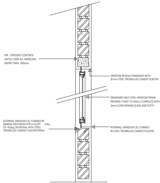
SECTION THROUGH WINDOW FOR 110 WALLS
