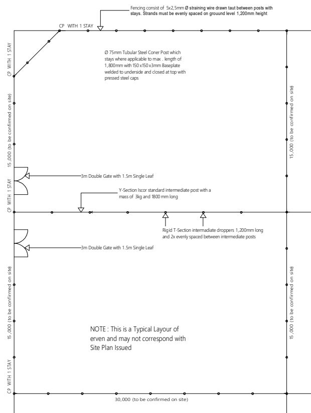
TYPICAL FENCING DETAILS
